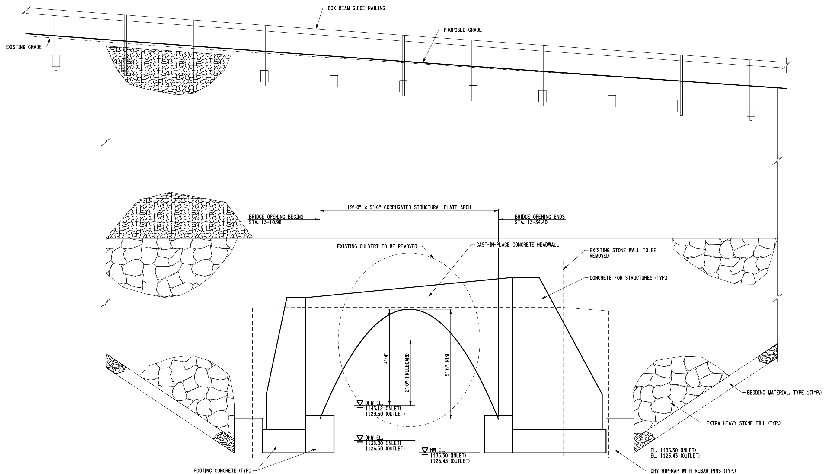
BRIDGE ELEVATION
