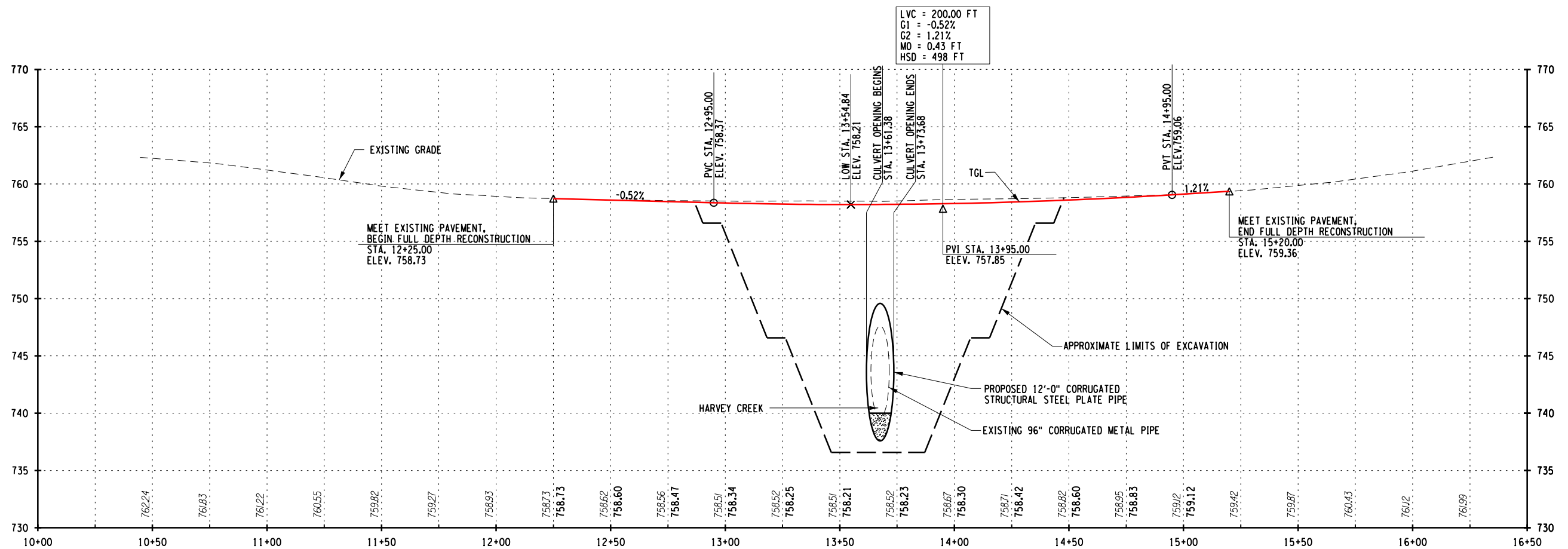
PINE GROVE ROAD (CR 39) PROFILE
