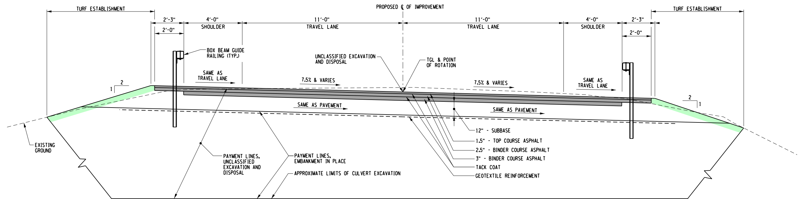
TYPICAL HIGHWAY SECTION FULL DEPTH RECONSTRUCTION (BANKED RIGHT)
