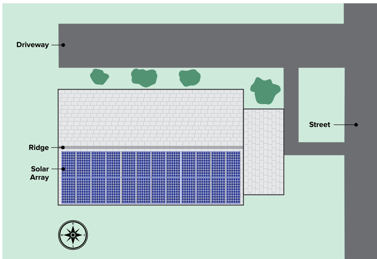
Typical single ridge structure where one or more exceptions apply (Figure 3)
